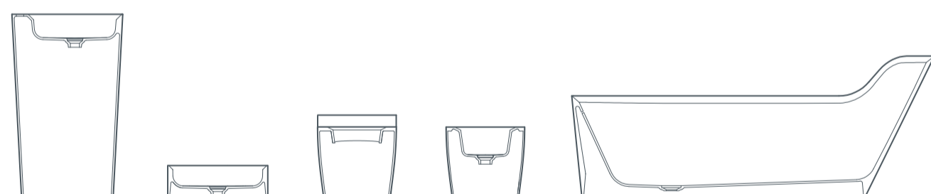
pearl washbasin freestanding 55x40x90 cm pearl washbasin countertop 50x40x15 cm pearl toilet wall hung 52x39x34 cm pearl bidet wall hung 52x39x34 cm pearl bath freestanding 182x81x70/50 cm
