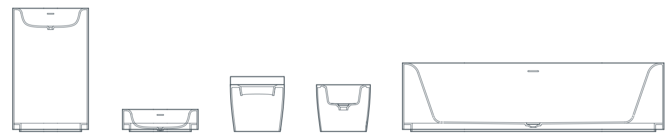
moon washbasin freestanding 55x45x90 cm moon washbasin countertop 55x45x16 cm moon toilet wall hung 52x39x34 cm moon bidet wall hung 52x39x34 cm moon bath freestanding 190x90x50 cm
